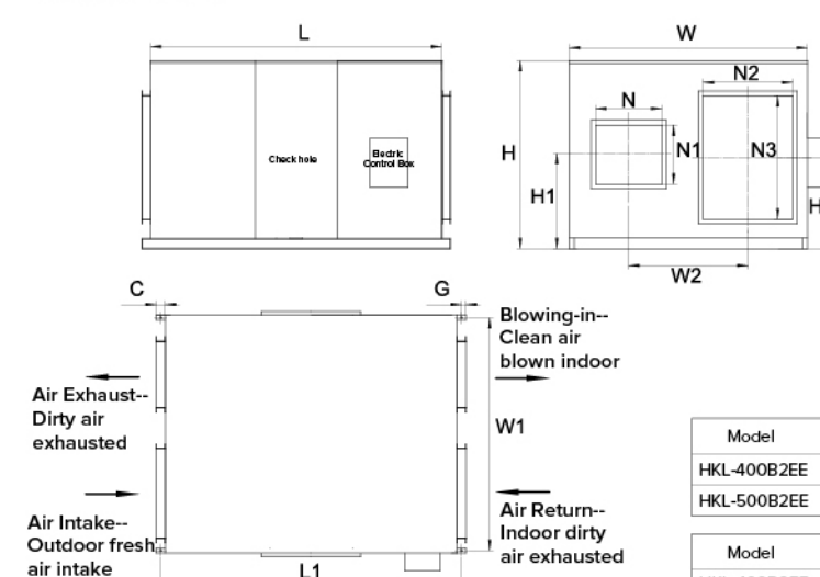
Product Dimensions
