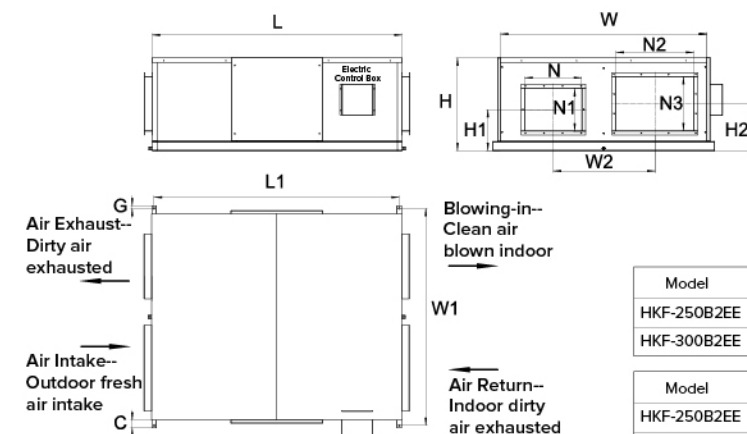
Product Dimensions
