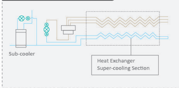
Two-stage Sub-cooling Cycle Diagram
